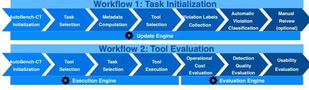
Figure 2: AutoBench-CT Workflow 1 and 2
