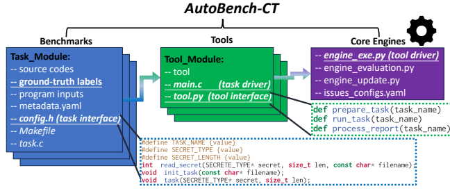
Figure 1: AutoBench-CT Architecture
